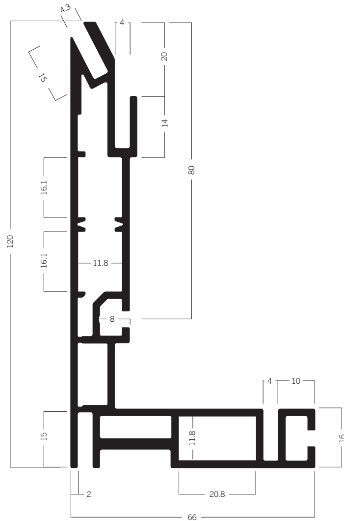
U 1060 Tension fabric extrusion 120 mm 16.20 kg | 6000 mm
