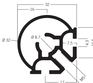
S 1200 Quarter-round extrusion 3.78 kg | 5000 mm
