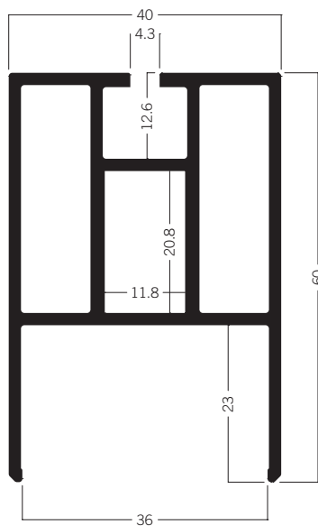
C 110 Beam extrusion 40 × 60 mm 7.57 kg | 6000 mm
