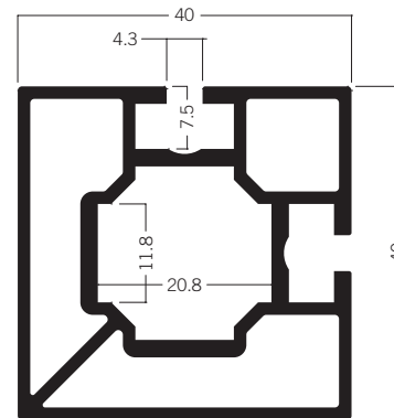
M 1007 Square extrusion 40 mm 7.17 kg | 6000 mm
