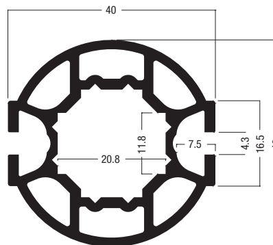
M 1202 Round extrusion 40 mm 6.10 kg | 5000 mm
