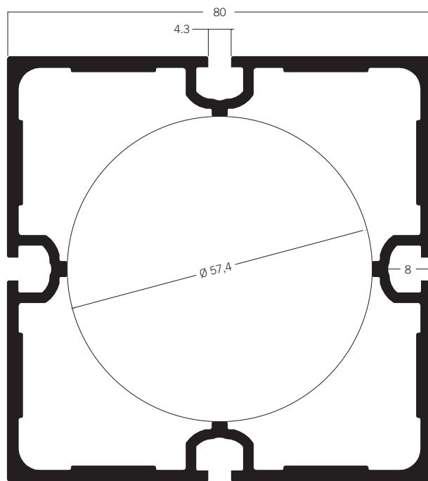
U 1020 Square extrusion 80 mm 15.50 kg | 6000 mm
