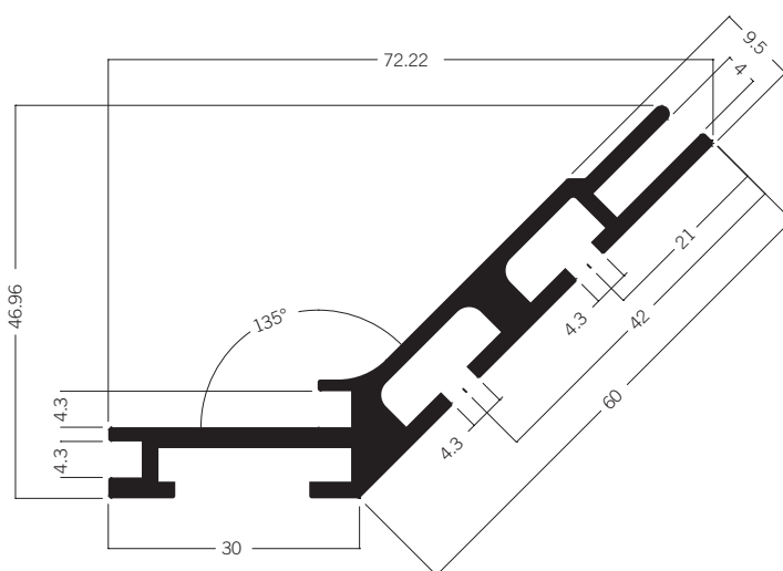
M 1301 Tension fabric extrusion 135° 6.55 kg | 6000 mm
