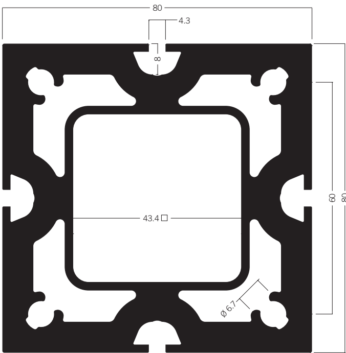
DFS 84 Upright extrusion 80 mm 38.95 kg | 5040 mm
