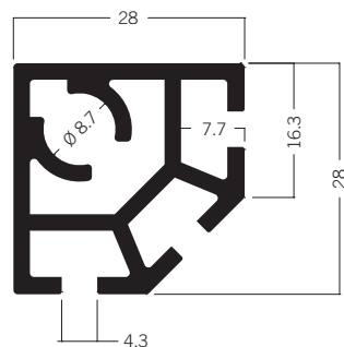
S 308 Upright extrusion 28 m 4.14 kg | 5000 mm
