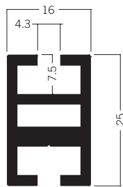
M 1602 Beam extrusion 25 mm 2.72 kg | 5000 mm
