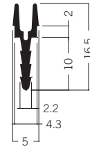
E 452 Extrusion connector 0.23 kg | 5000 mm
