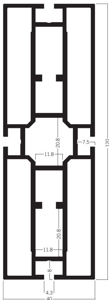
M 1031 Rectangular extrusion 120 mm 18.07 kg | 6000 mm
