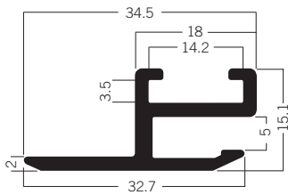
C 875 Frame extrusion 34.5 × 15 mm 2.22 kg | 6000 mm
