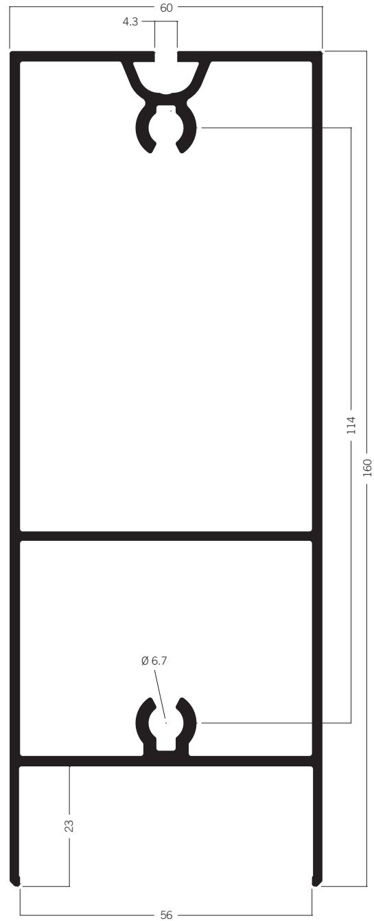
C 316 Door beam extrusion 60 x 160 mm 18.12 kg | 6000 mm
