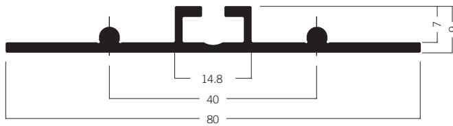
WP 830 Cover extrusion for extrusions 80 mm 3.58 kg | 6060 mm
