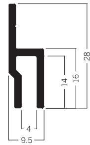
M 1614 Tension fabric extrusion 28 mm 1.54 kg | 6000 mm
