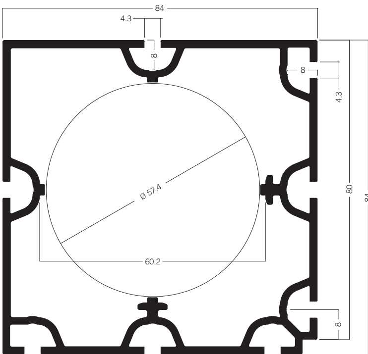
DFS 84/6000 Upright extrusion 80 mm 46.28 kg | 6000 mm
