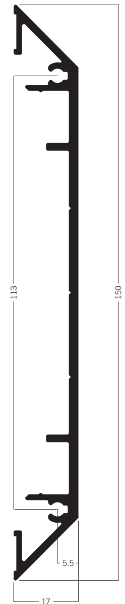
C 1327 Cable channel extrusion 7.23 kg | 6000 mm
