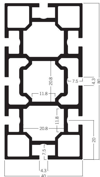
M 1092 Rectangular extrusion 80 mm 14.60 kg | 6000 mm
