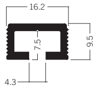
W 416 Insert extrusion 16 mm 1.05 kg | 5000 mm
