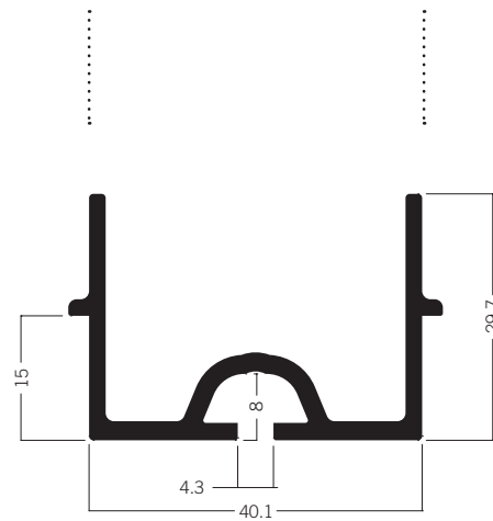
M 1155 Cover extrusion for M 1059 3.46 kg | 5000 mm
