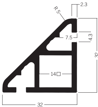
S 1302* Triangular extrusion 32 mm 3.20 kg | 5000 mm
