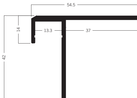
SO 630 Skirting extrusion for LED module 3.20 kg | 5000 mm
