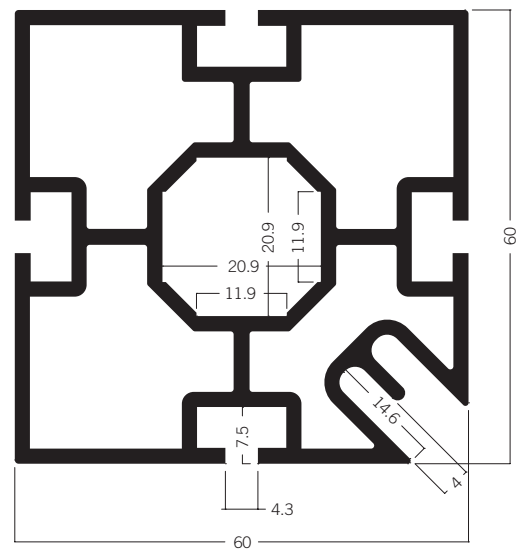
S 385R* upright extrusion, with silicone edge groove (USA) 14.01 kg | 6150 mm
