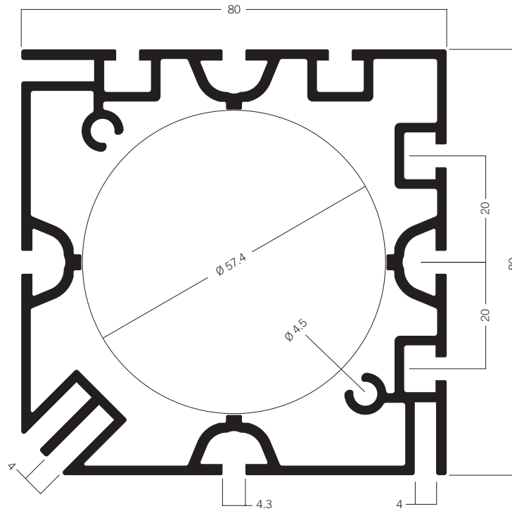
WP 850 Upright extrusion 90°, with silicone edge groove 16.48 kg | 6000 mm
