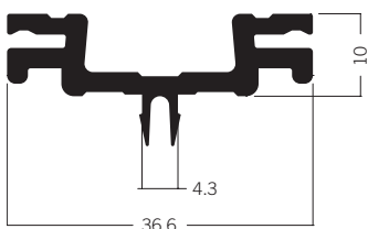
C 160 Adaptor extrusion 10 × 37 mm 1.61 kg | 6000 mm
