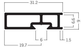
C 722 Retainer extrusion 31 × 9 mm 1.83 kg | 6000 mm
