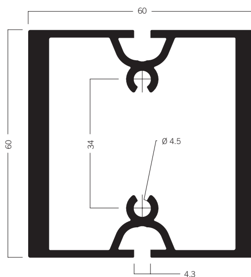
C 60-125 Upright extrusion 60 x 60 mm 16.25 kg | 6000 mm
