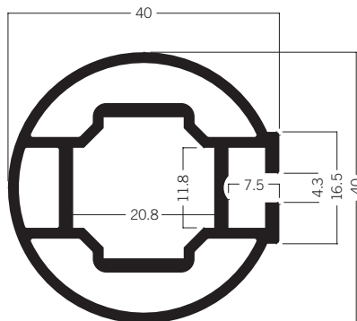
M 1201* Round extrusion 40 mm 5.25 kg | 5000 mm
