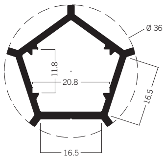
M 1980 Luminous elements extrusion 2.65 kg | 5000 mm
